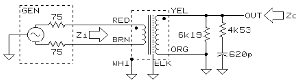
TEST CIRCUIT 1
