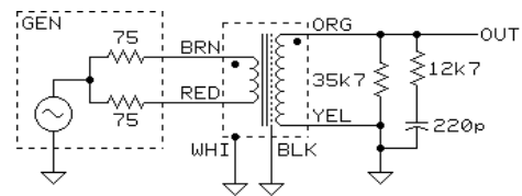
TEST CIRCUIT 2
