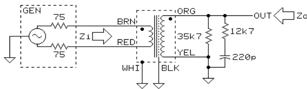
TEST CIRCUIT 1
