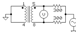
TEST CIRCUIT 2
