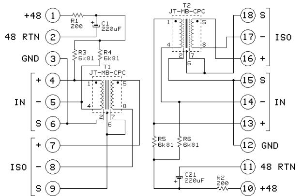
Onboard provisions allow local 48V phantom power to the connectors
