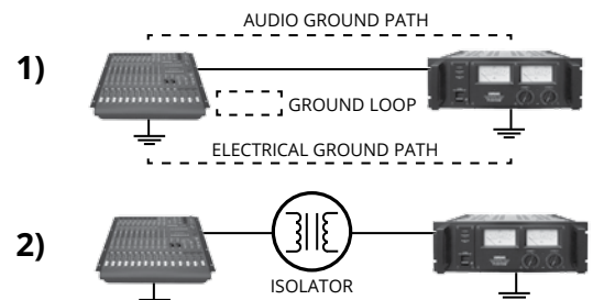
Lifting the ground and passing the signal through the transformer totally eliminates the ground loop
