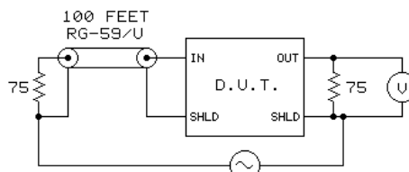
TEST CIRCUIT 2
