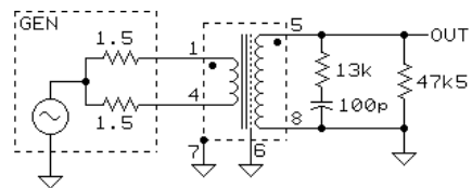
TEST CIRCUIT 2
