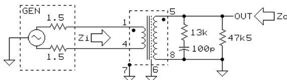
TEST CIRCUIT 1
