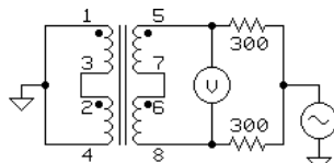
TEST CIRCUIT 2
