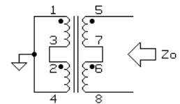
TEST CIRCUIT 4
