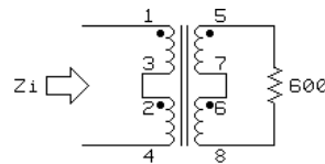
TEST CIRCUIT 3
