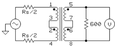
TEST CIRCUIT 1
