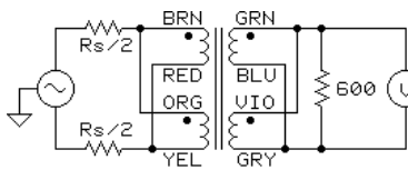
TEST CIRCUIT 1
