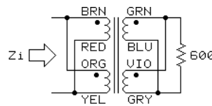
TEST CIRCUIT 3
